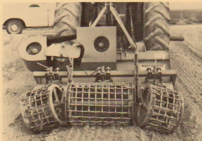
A close up of a one row tiller with mesh rollers.
